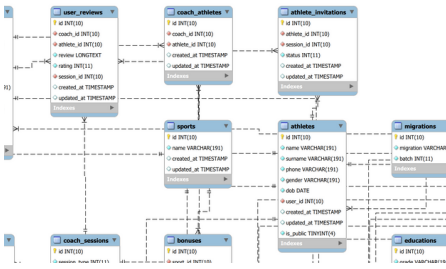
Example of Database Design
